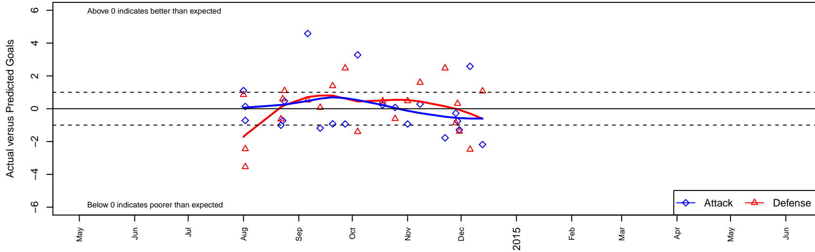
NSC Spark G03 Dots are actual minus expected GF (blue circles) and GA (red triangles). Blue line is smoothed change in attack strength. Red is smoothed change in defense strength.
